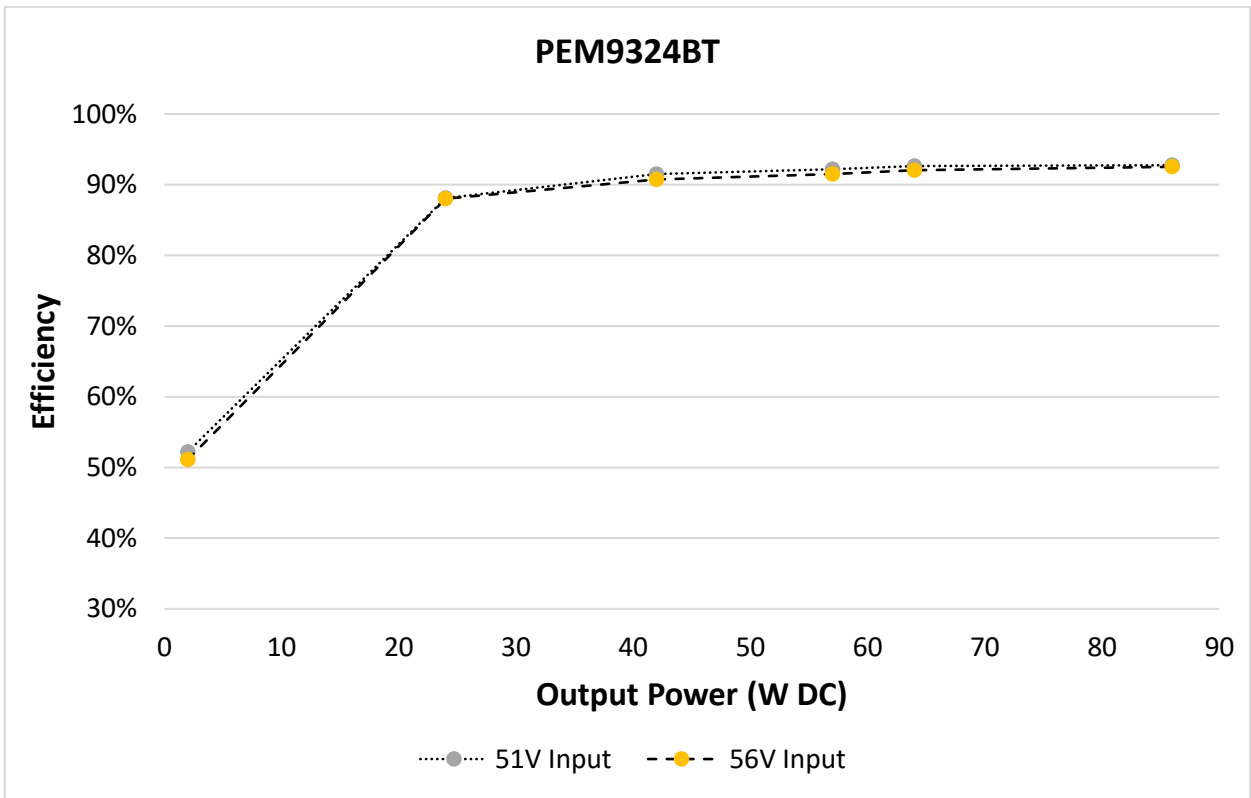
Figure 6- PEM9324BT Efficiency vs. Output power end to end
