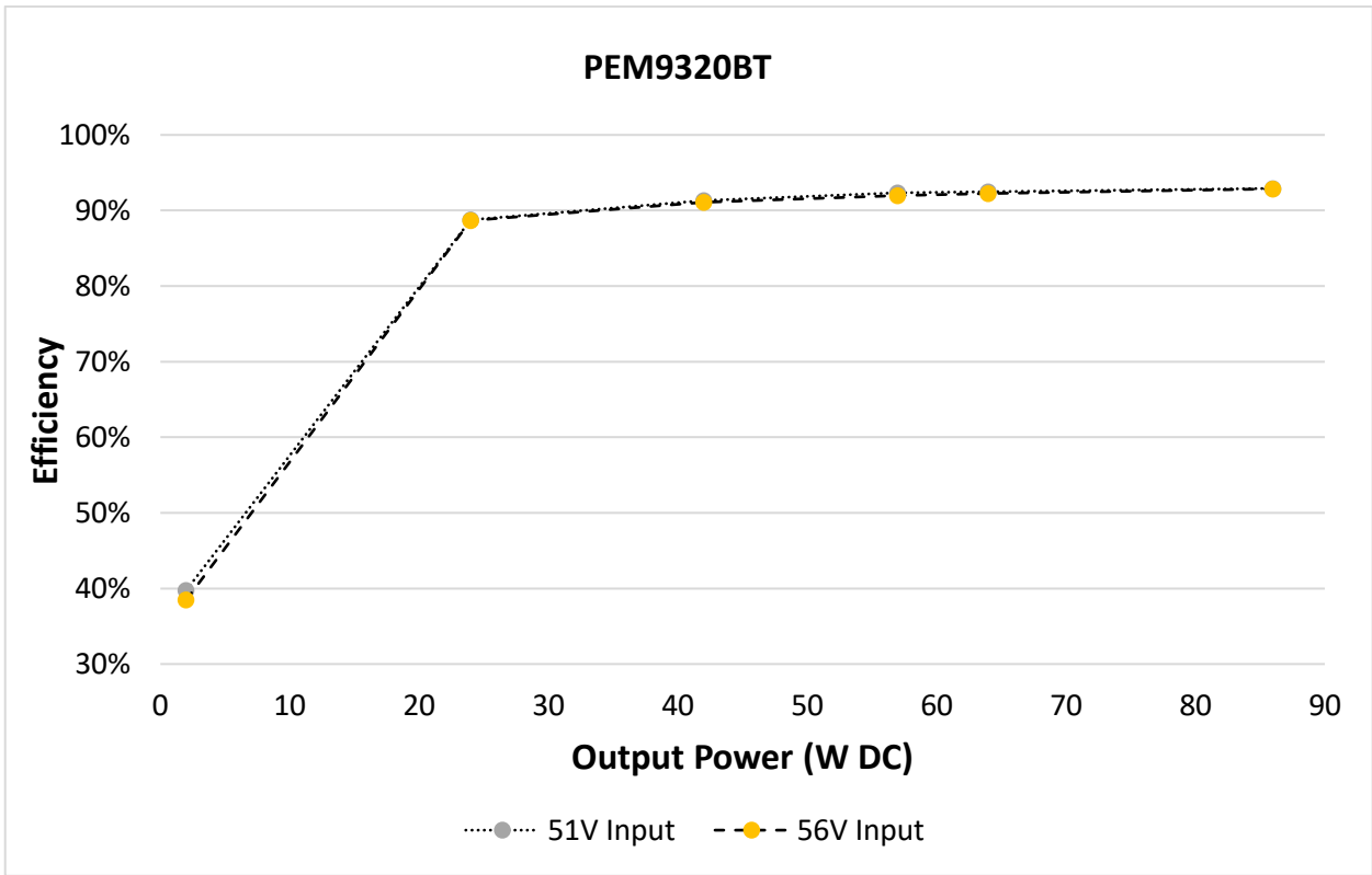
Figure 5- PEM9320BT Efficiency vs. Output power end to end
