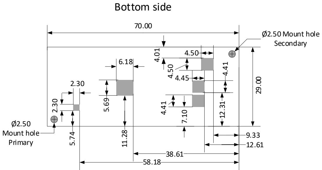
Figure 8- Thermal pad diagram
