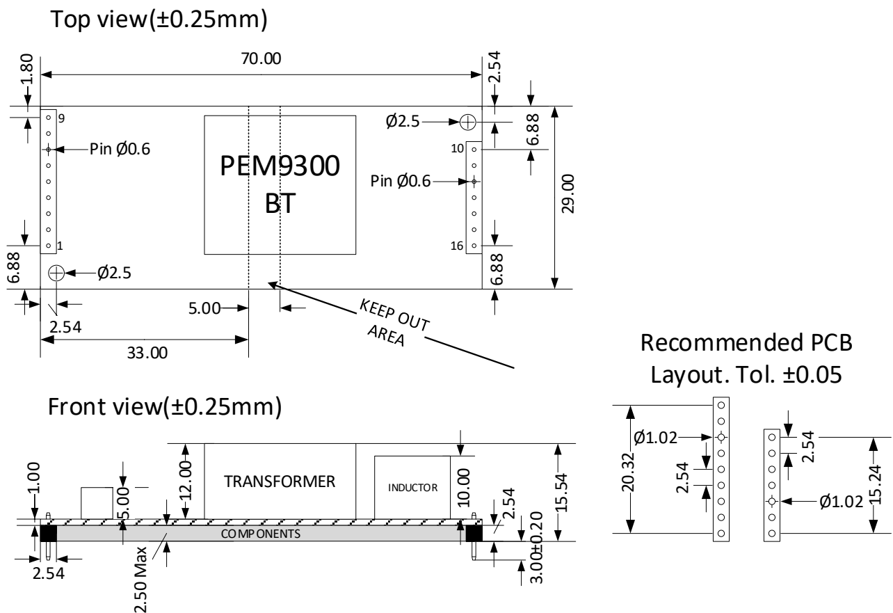
Figure 9- Mechanical Dimensions
