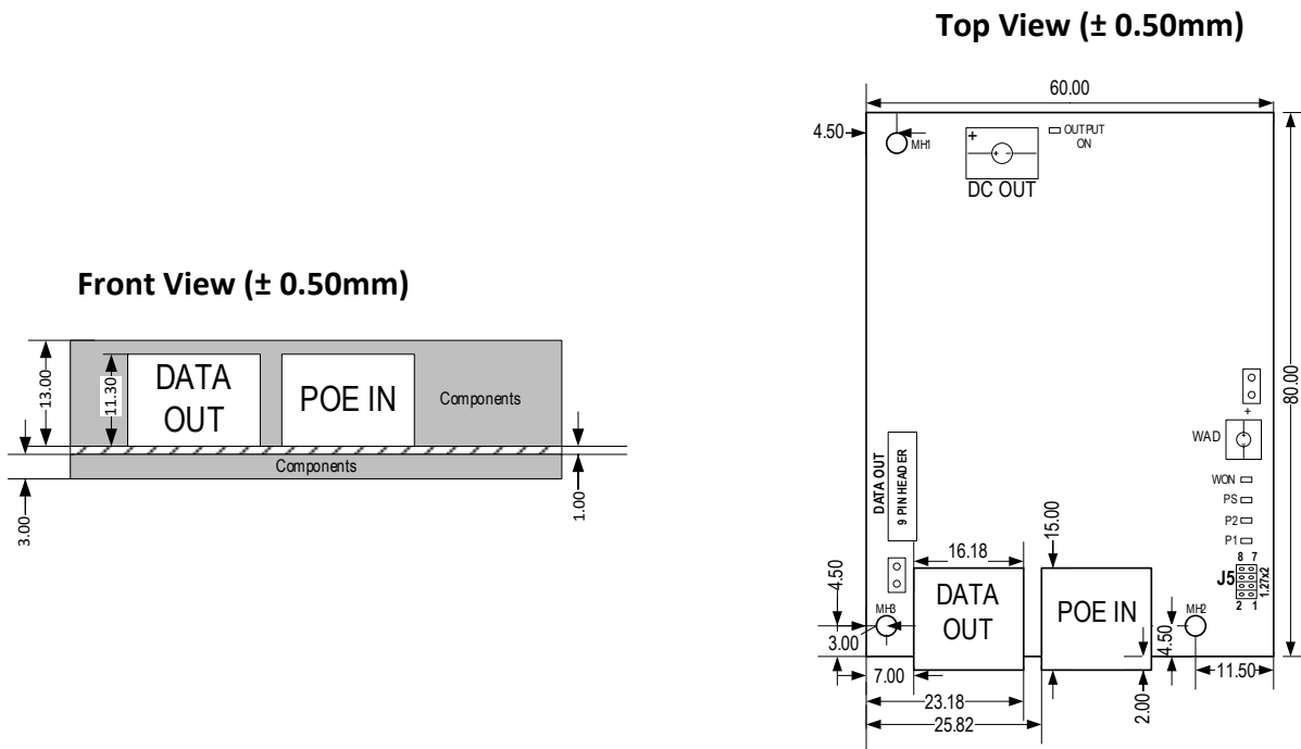
Figure 4- Mechanical Dimensions
