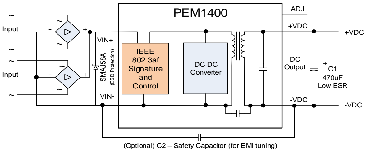
Figure 3- Block Diagram
