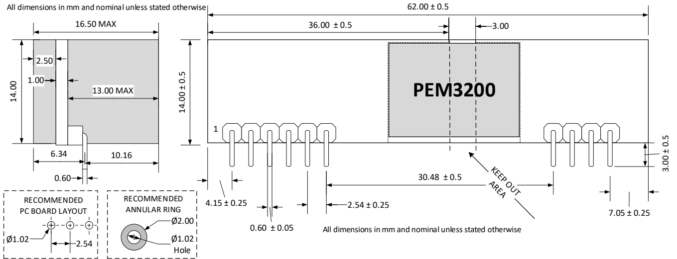
Figure 9- Mechanical Dimensions
